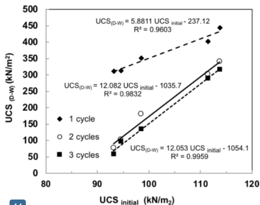
Fig. 7. Relationship between UCS_{initial} and UCS_{(D-W \text{ cycles})}
